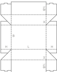
0440 | A
